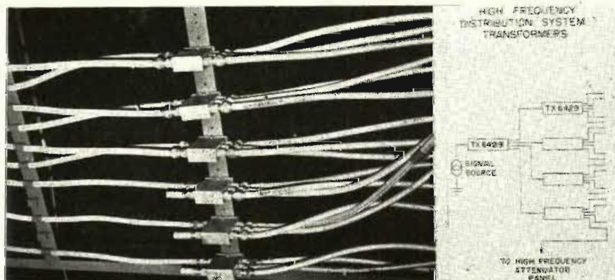
Figure 12 High-frequency distribution system transformers.
