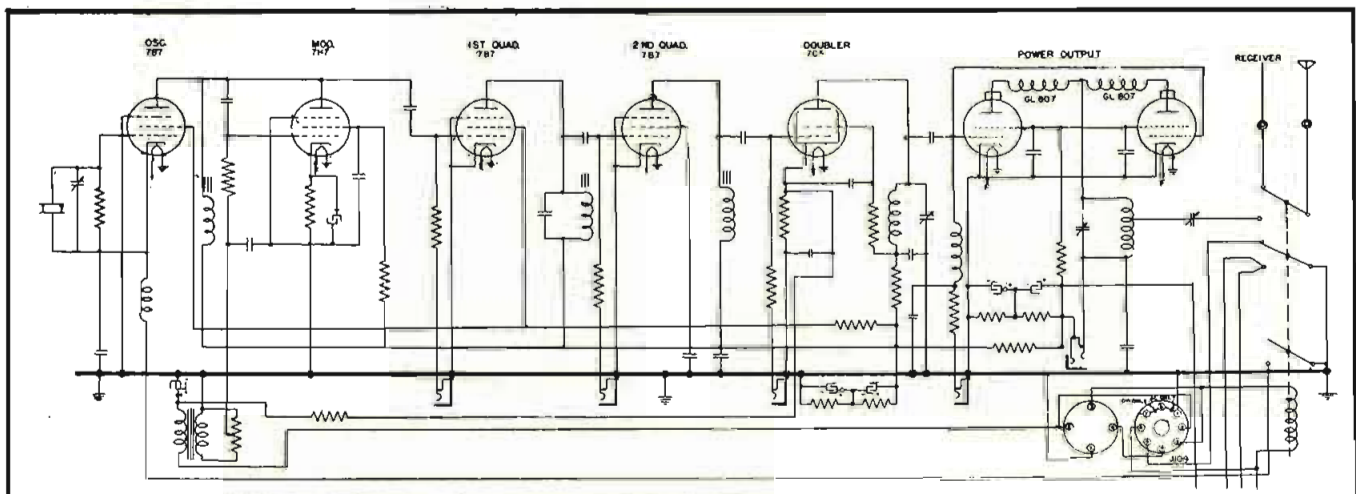
Figure 7 Transmitter schematic.
