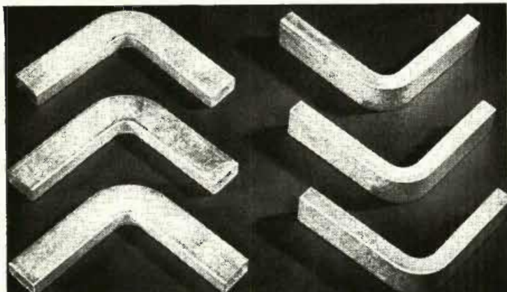
Figure 1 Rectangular aluminum waveguide tubes, 1" x .05"
