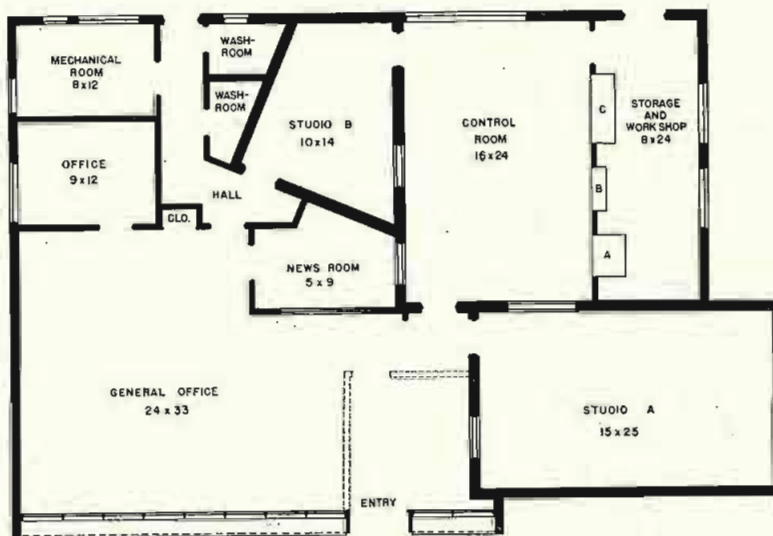
Layout for 1 kw a-m (A) and 1 kw f-m (C) system. In B of this layout we have the rooms for audio and test equipment. This is a setup used at KSJO, San Jose, Calif., where John G. Bauriedel is engineering director and Larry King is chief engineer.
