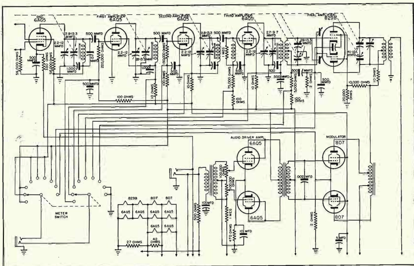
Schematic of the v-h-f transmitter. Crystal switching unit similar to that shown on the receiver diagram is used in this transmitter.
